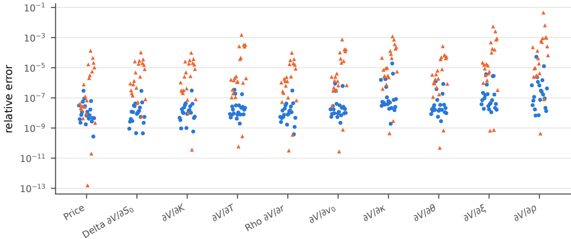
Heston AAD engine, 21 parameter sets (Q32.32 RTL simulation)
